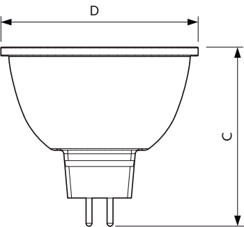
MR16 12V 7-35W 400lm 25D 3000K GU5.3 D
