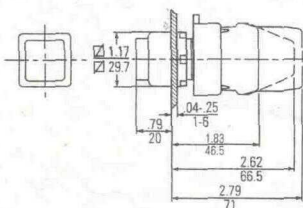
Square Illuminated Extended Push Button
