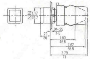
Square Illuminated Flush Push Button
