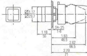
Square Illuminated Recessed Push Button
