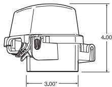
SINGLE GANG COVER
