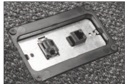
Single-Gang WMFB Box with Single Receptacle and one Communication Port.
