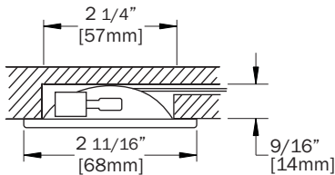
514 580 Recessed Mount
