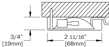
514 585 Surface Mount
