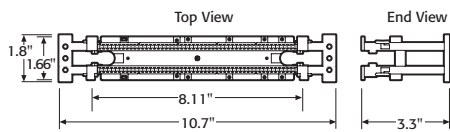
50-Pair Wiring Block (with legs)
