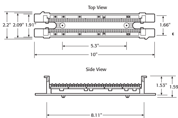
50-Pair 89D Bracket Compatible Wiring Block
