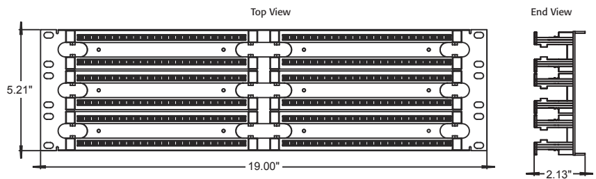
300-Pair Rack-Mount Wiring Block
