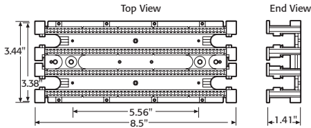
100-Pair Wiring Block (without legs)
