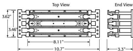
100-Pair Wiring Block (with legs)
