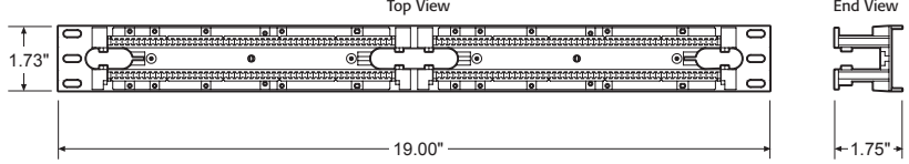
100-Pair Rack-Mount Wiring Block
