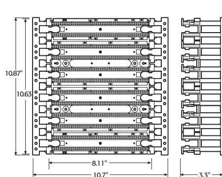
300-Pair Wiring Block (with legs)
