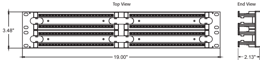
200-Pair Rack-Mount Wiring Block
