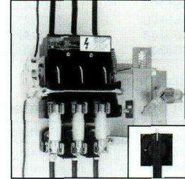
Type MCS Disconnect Switch with rotary handle
