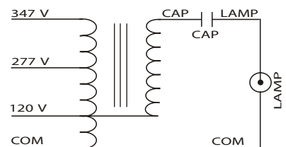
120/277/347 VOLT CONNECTION
