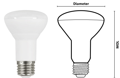
MOL : 3 13/16 in. (97 mm) Dia. : 2 15/32 in. (63 mm)
