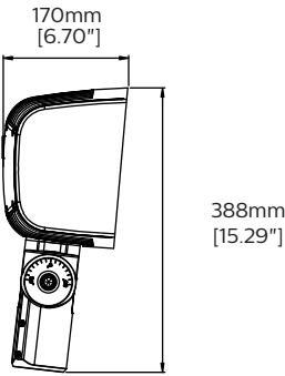
FL150 and FL200-S Side
