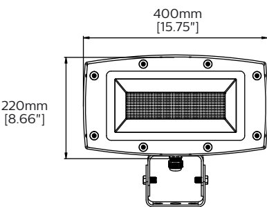
FL150-T and FL200-T Front
