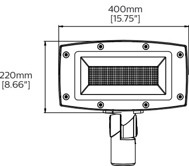
FL150 and FL200-S Front
