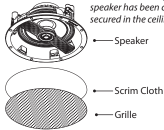
Speaker Assembly
