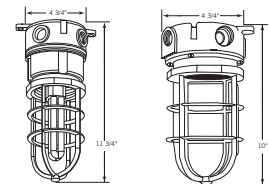
ceiling mounts
