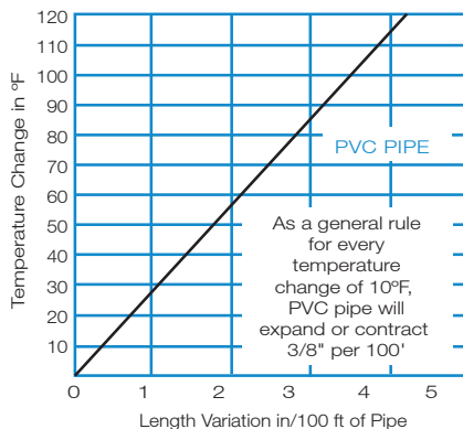
PVC Pipe Length Variation due to Temperature Change (°F) Coefficient = 3.6 \times 10^{-4} in/ft/°F
