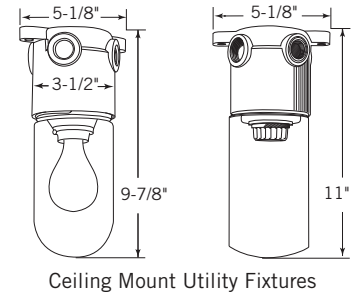
Ceiling Mount Utility Fixtures
