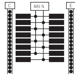
TLM1615CCU, TM1615RCU, TLM1620CCU, TLM1620RCU
