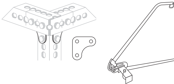
RA-GP Gusset Plate For extra rigid assembly
