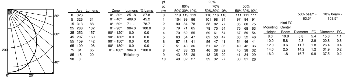
WF6 SQ B LED 30K40K50K _ 4000K LED's , input watts: 12, delivered lumens: 904, LM/W=75, test no. ISF 36826P41
