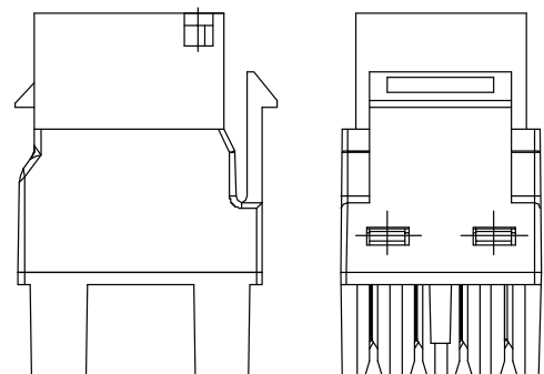
Cat6 180° Keystone
