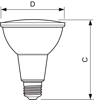
12PAR30L/AMB/F40/830/DIM ULW
