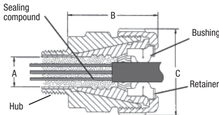
With bushing
