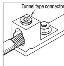
TUNNEL TYPE CONNECTOR TERMINATION LOAD AND LINE
