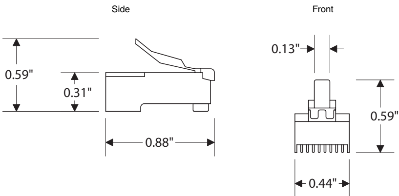
47613-EZC - EZ-RJ45 Connector
