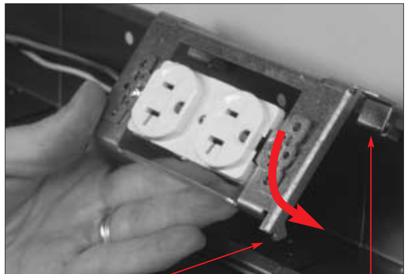
Rotate Bracket down and snap into place.
