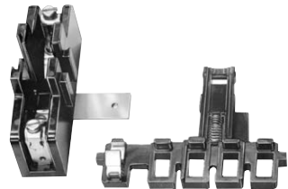
Fifth-pole kit
