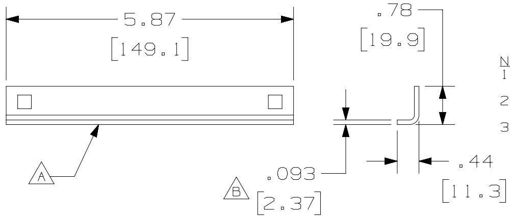
EXPANSION SPLICE BRACKET
