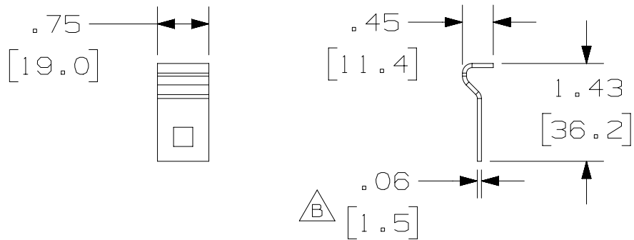
EXPANSION SPLICE CLIP
