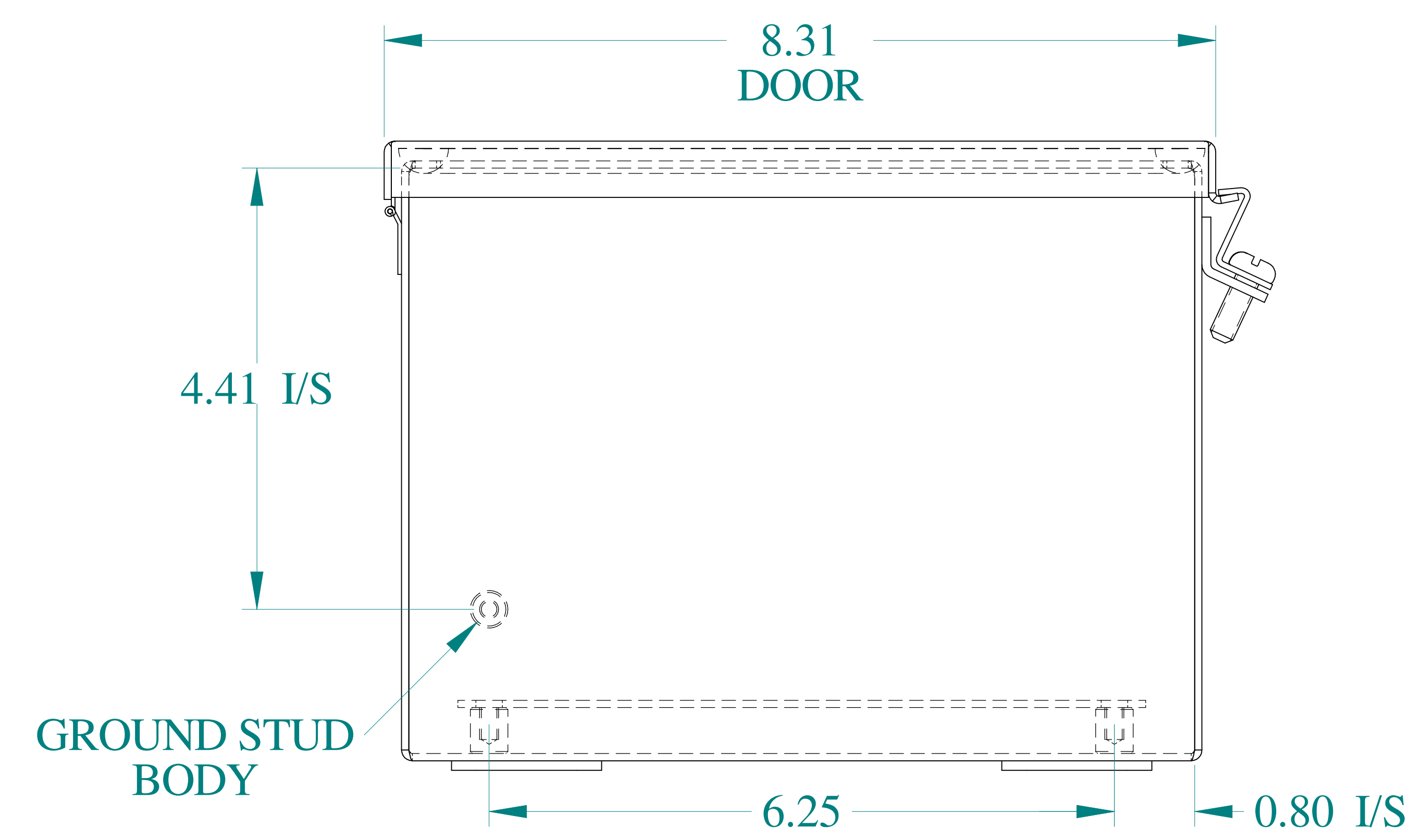
BOTTOM VIEW
