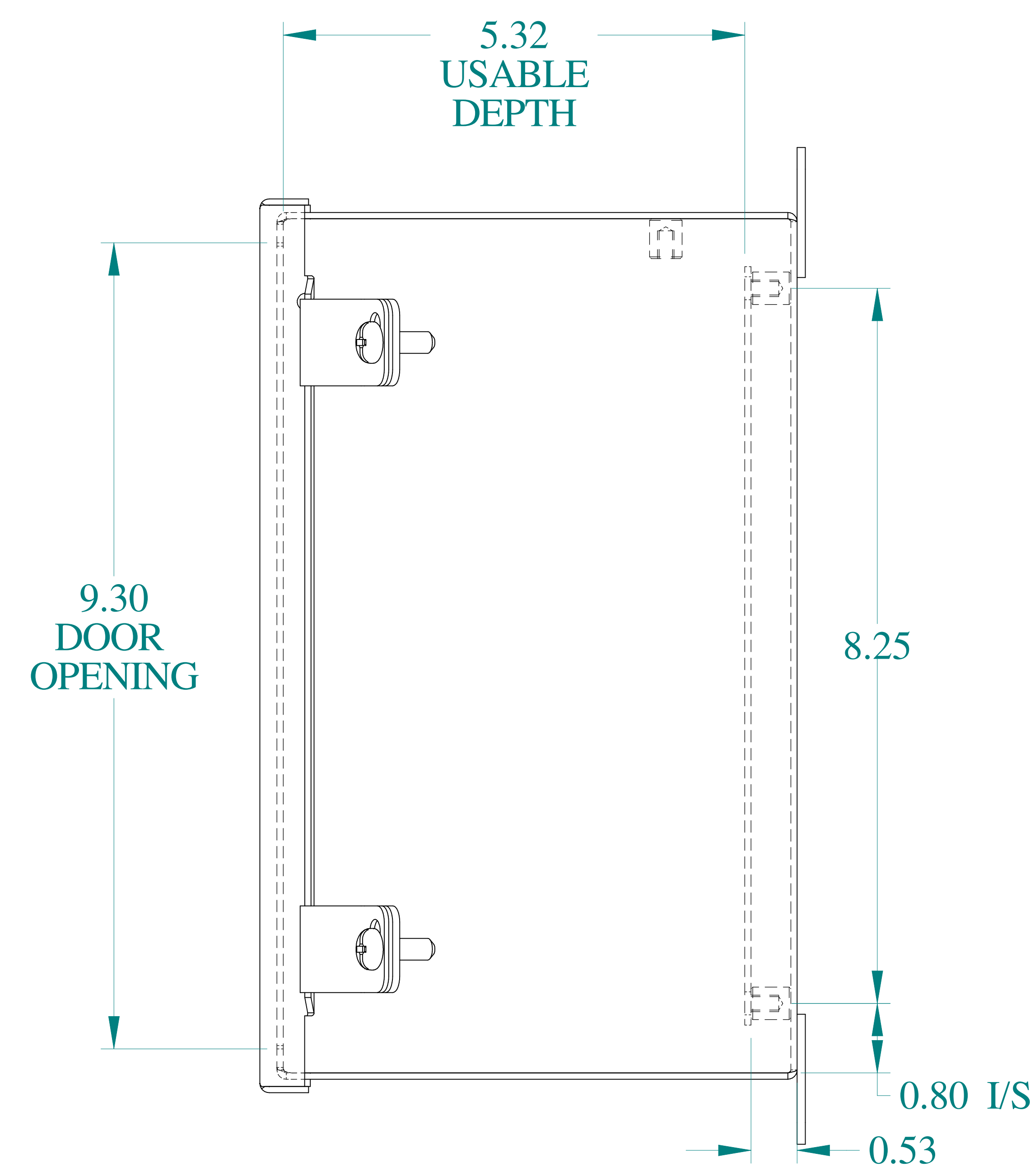
SIDE VIEW
