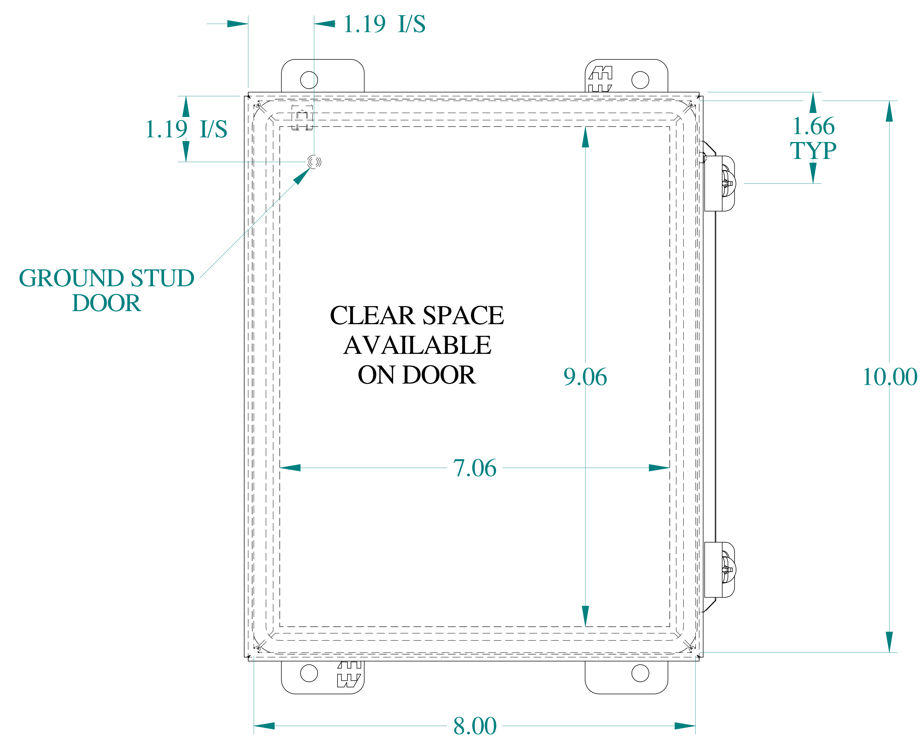
FRONT VIEW
