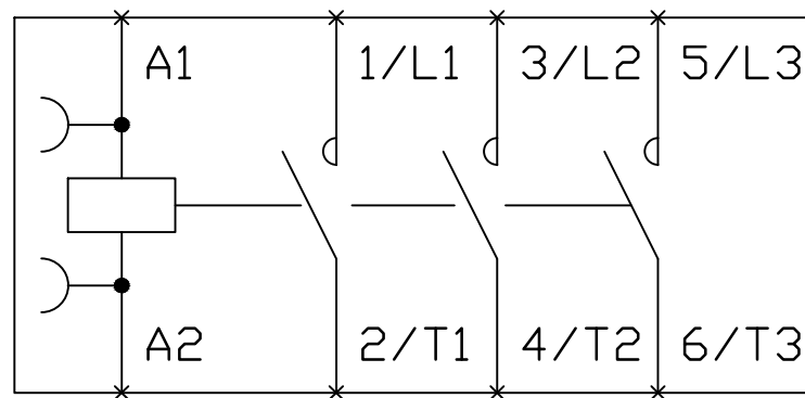
LEN00D & E Wiring Diagram
