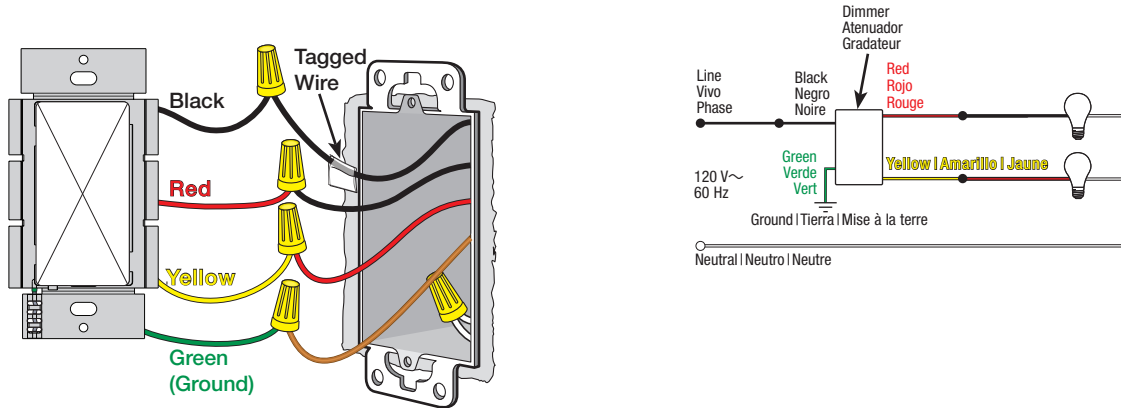
Image #72 — Dual Control with One Black Wire, One Red Wire and One Yellow Wire in a Single Pole Application
