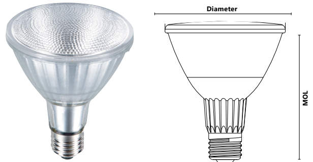
MOL: 4 21/32" (118 mm) Dia.: 3 3/4" (95 mm)
