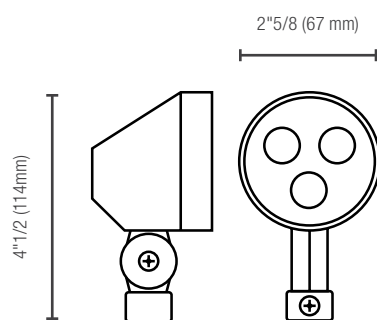
Type N - PAR18 Thermoplastic
