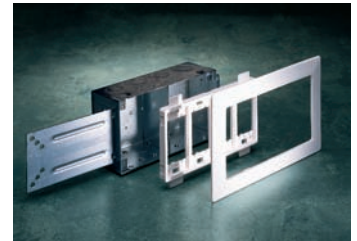
Behind the low-profile exterior of WallSource lies a rugged in-wall box with more than enough room for all your wiring needs.
