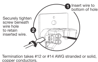
Screw Pressure Plate Back Wire
