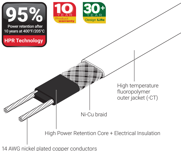
Heating Cable Construction
