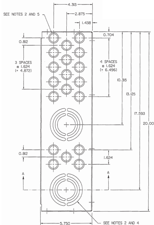
EWK1 End Wall w/KOs (20"W X 5.75"D)
