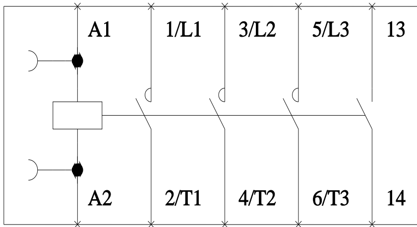
LEN00B03 Wiring Diagram
