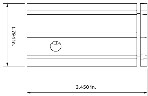
Welding mold
