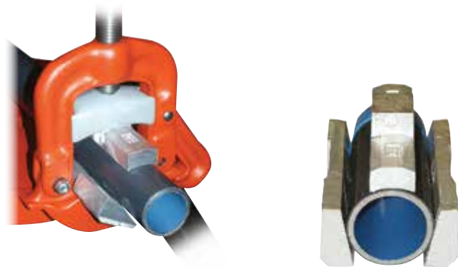
Ocal jaws for PVC-coated conduit
