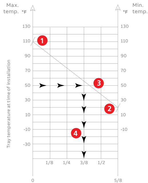
Figure 1 - Proper gap settings
