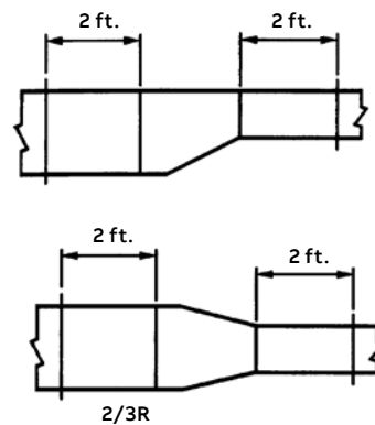
Horizontal reducer
