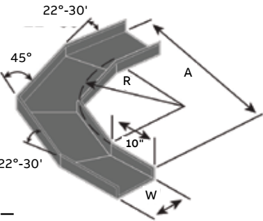
Horizontal bends
