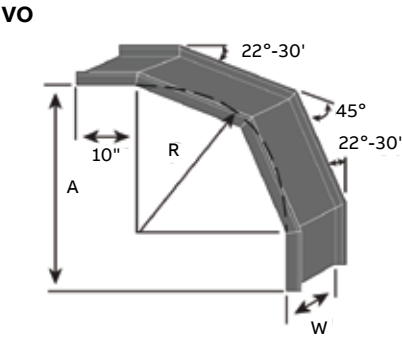
Vertical bends
