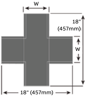
Horizontal crosses
