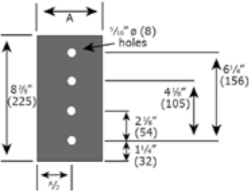
Standard splice plates
