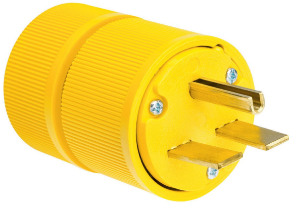
Gator Grip Plug, 2 pole 3 Wire, 30A 250V Grounding, Yellow
