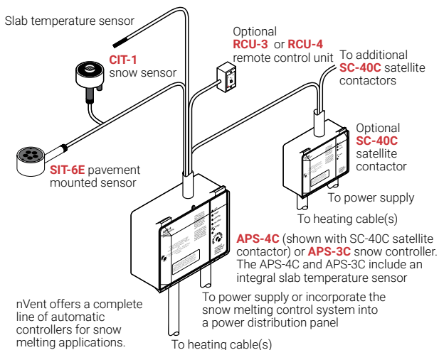
Figure 36: Automatic snow melting control system
