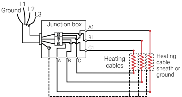
Figure 38: Typical 3Ø Delta connection
