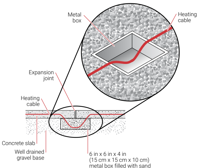
Figure 10: Crossing expansion joints
