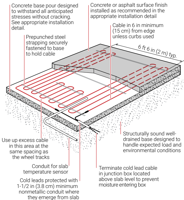
Figure 23: Wheel track installation detail
