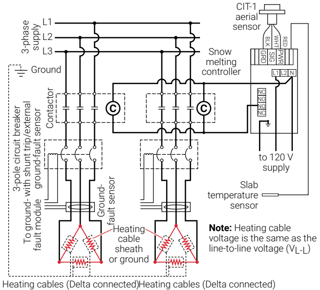
Figure 45: Control of balanced 3Ø Delta connected heating cables with individual contactors and APS-3C automatic snow controller
