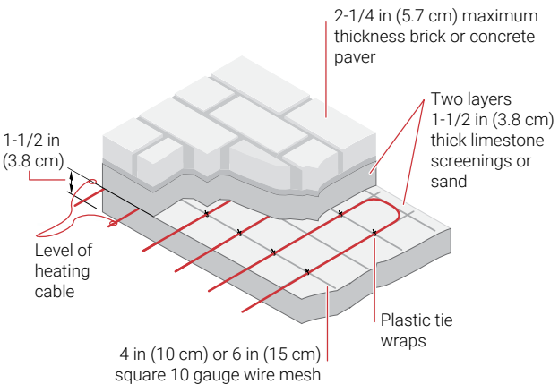
Figure 21: Cross-section showing material layers for paver area
