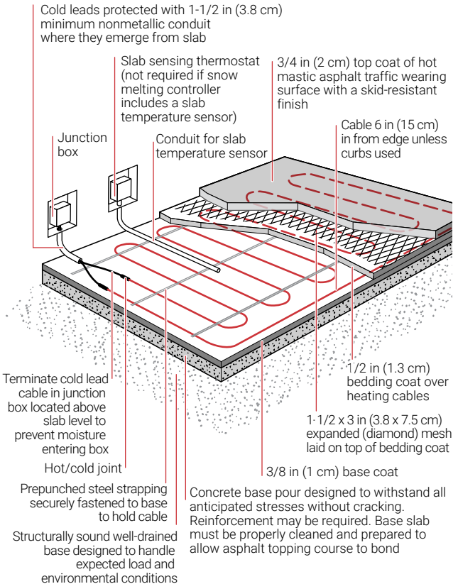
Figure 20: Mastic asphalt with concrete base
