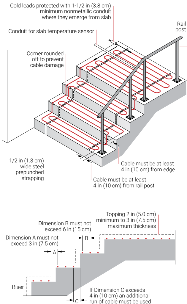
Figure 24: Stair installation detail
