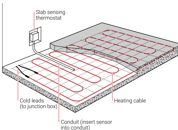
Figure 35: Slab sensing thermostat installation
