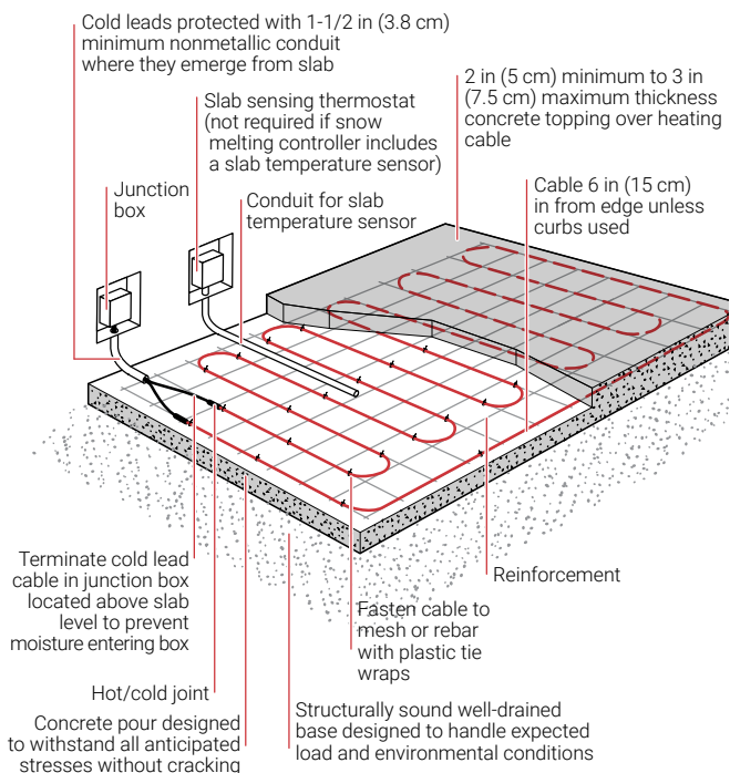
Figure 14: Single-pour concrete
