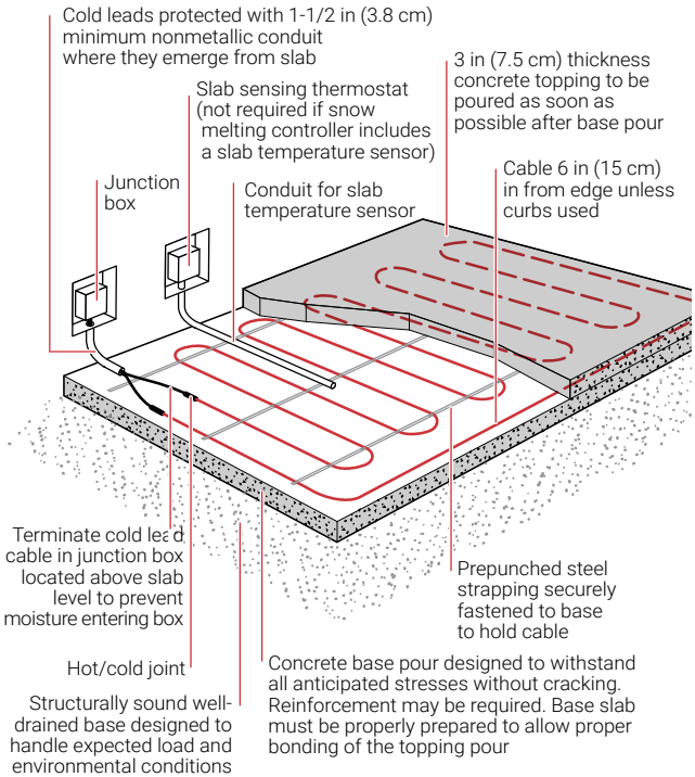
Figure 15: Two-pour concrete
