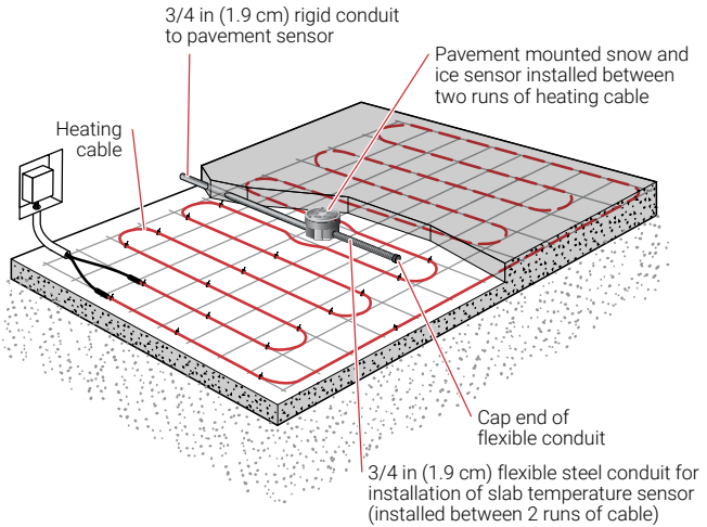
Figure 13: Alternative slab temperature sensor installation
