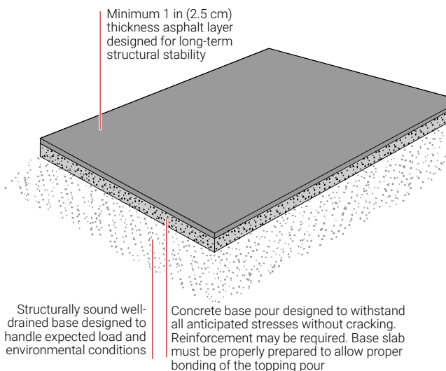
Figure 17: Asphalt installation with concrete base
