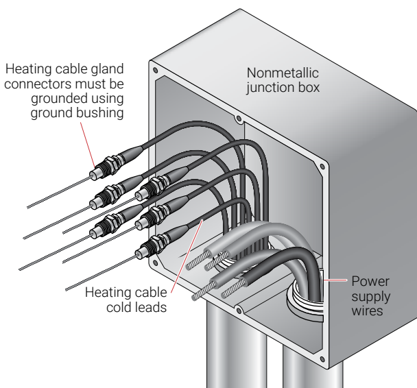
Figure 31: Nonmetallic junction box mounted on wall
