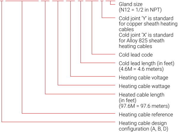
Figure 3: MI heating cable catalog number
