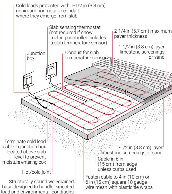
Figure 22: Brick and concrete pavers
