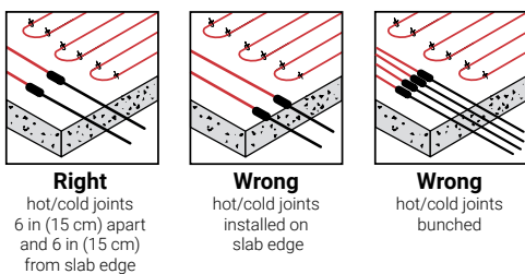
Figure 7: Positioning hot/cold joints
