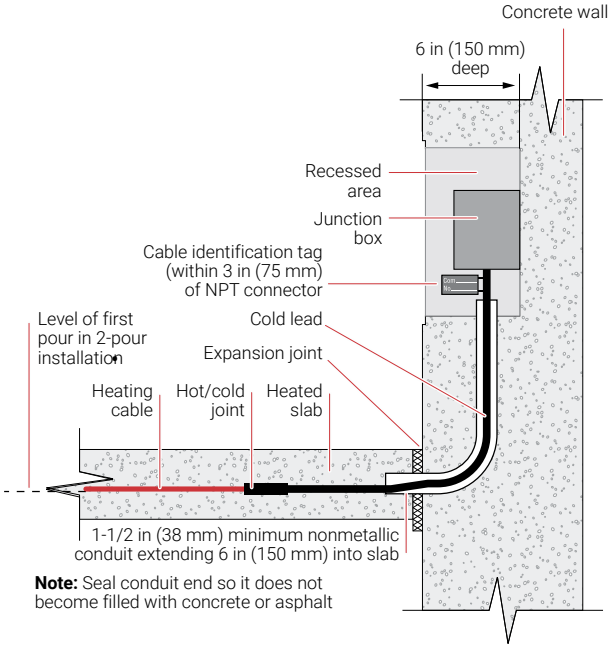
Figure 26: Junction box recessed in wall
