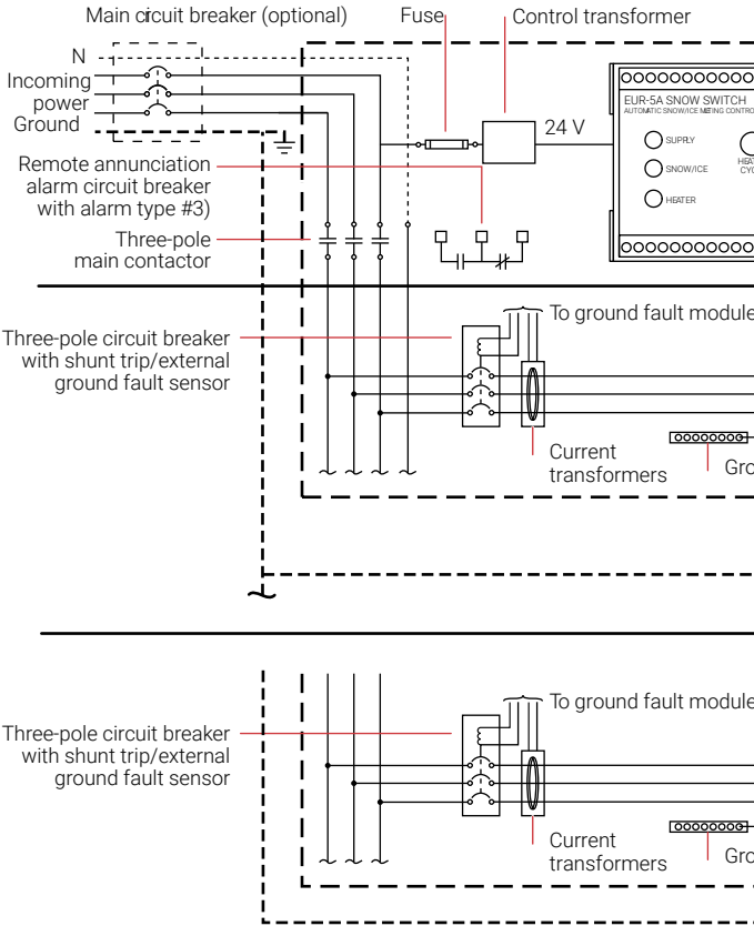
Figure 47: SMPG3 power distribution and control panel
