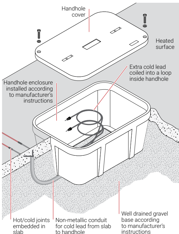
Figure 33: Handhole enclosure mounted in concrete slab
