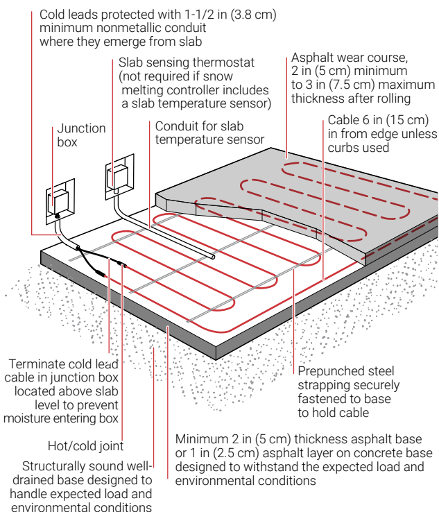
Figure 18: Asphalt installation
