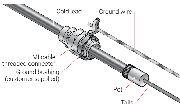
Figure 32: Using ground bushing to ground heating cable sheath
