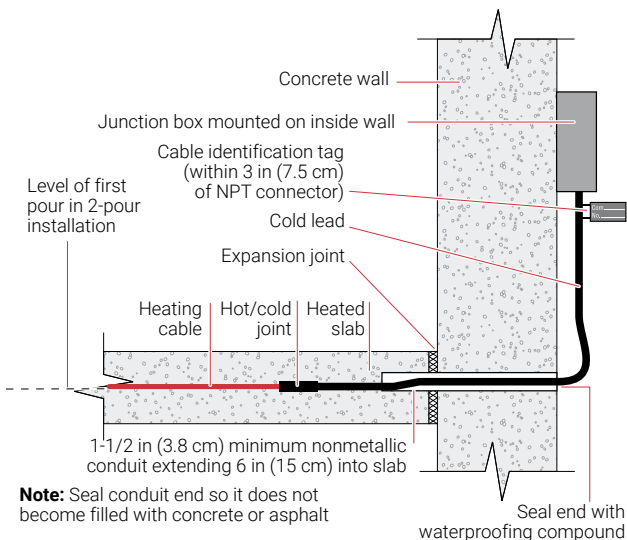
Figure 27: Junction box mounted on inside wall
