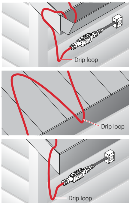
Figure 25: Drip loops
