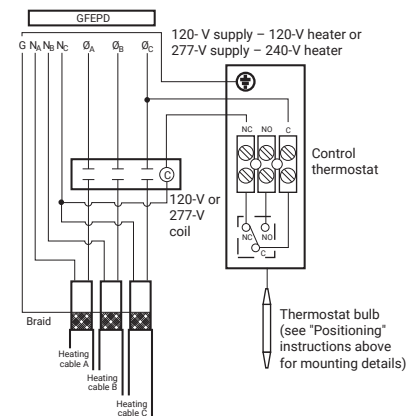
Figure 4. Contactor control
