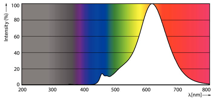
Spectral Power Distribution Colour - 5ST19/VIN/820/E26/CL/GL/DIM 4/1FBH T20
