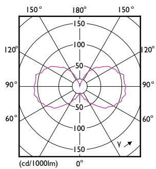
Light Distribution Diagram - 5ST19/VIN/820/E26/CL/GL/DIM 4/1FBH T20
