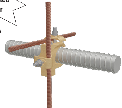
Rebar Connection
