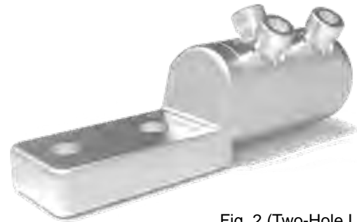
Fig. 2 (Two-Hole Lug)
