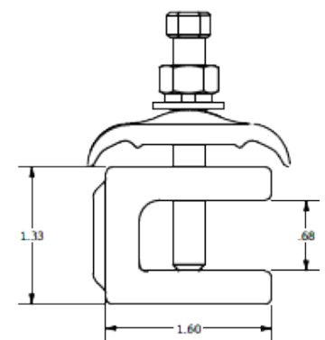
Line Art dimensions shown are GCS26HEX connector
