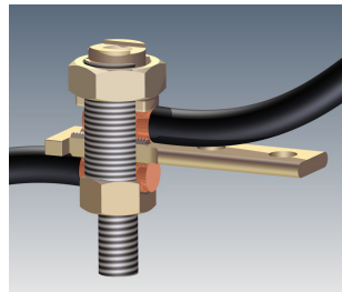
Splice Connection
