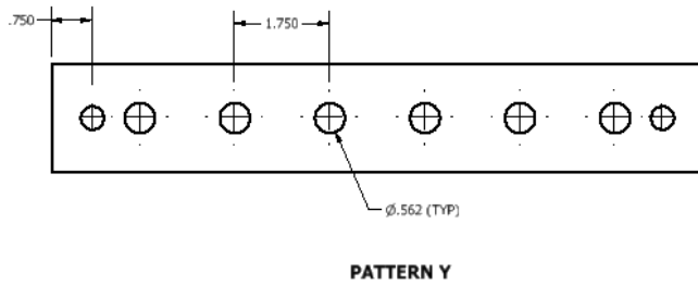
Single row of NEMA holes
