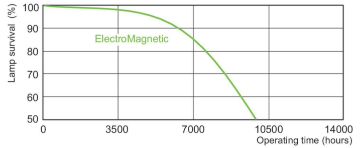
Life Expectancy Diagram - PL-S 13W/850/2P 1CT/5X10BOX ALTO
