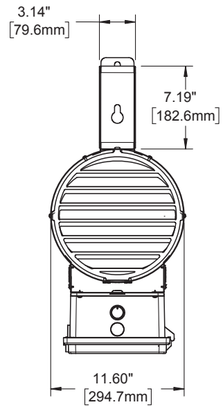
DEVANT | FRONT
