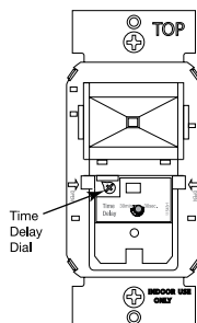
Fig 6: Time Delay Adjustment
