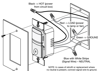
Fig 4: Sensor orientation, wire connections and wall box assembly
