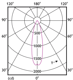
Light Distribution Diagram - 5.5PAR20/COR/F25/927-922/DIM/P/T20 6/1FB
