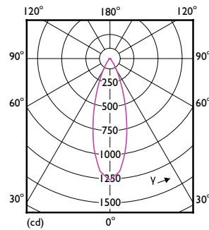
Light Distribution Diagram - 5.5PAR20/LED/F40/930/DIM/G/T20 6/1FB
