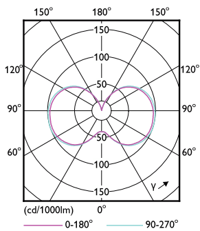
Light Distribution Diagram - 150CC/LED/840/ND EX39 G2 BB 3/1
