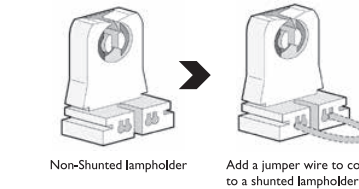
Figure showing how to convert a non-shunted lampholder to a shunted lampholder using a jumper wire.
